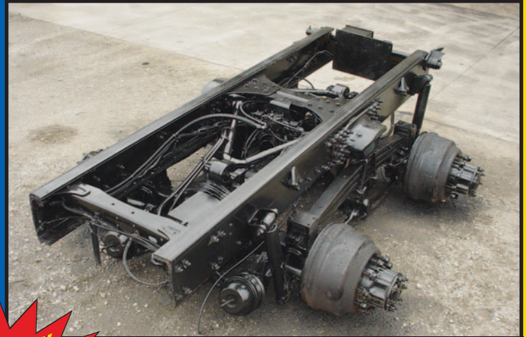
Rockwell RT46-160C Locker cutoff 4.63 ratio
